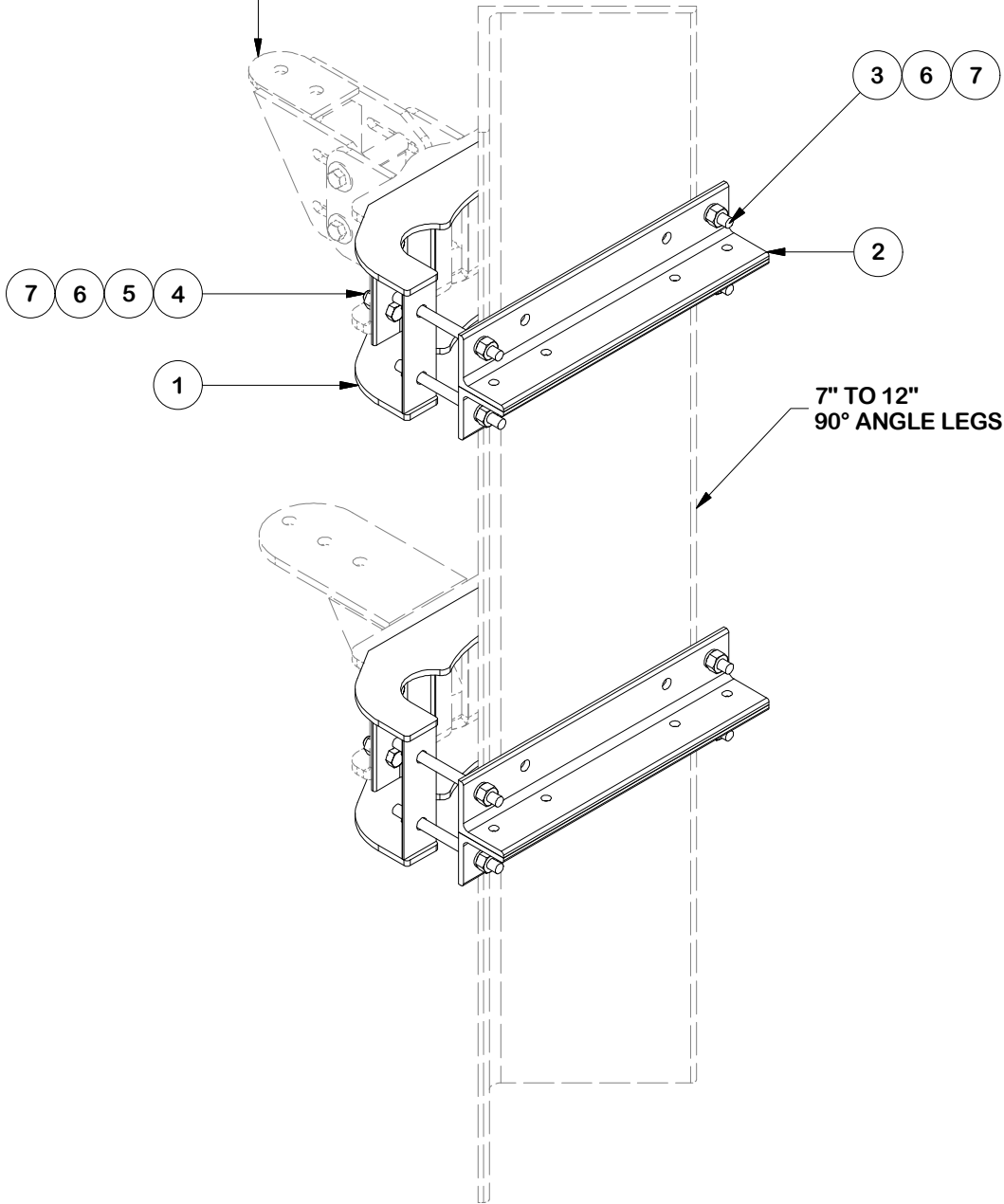
ANGLE LEG CONNECTION
