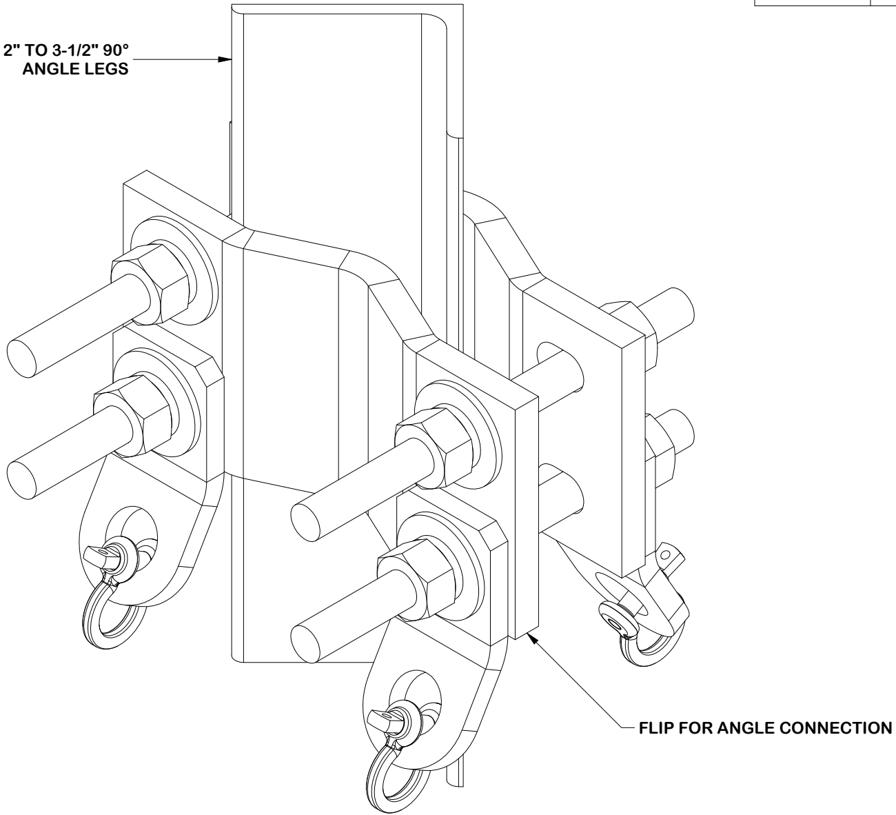
ANGLE LEG CONNECTION
