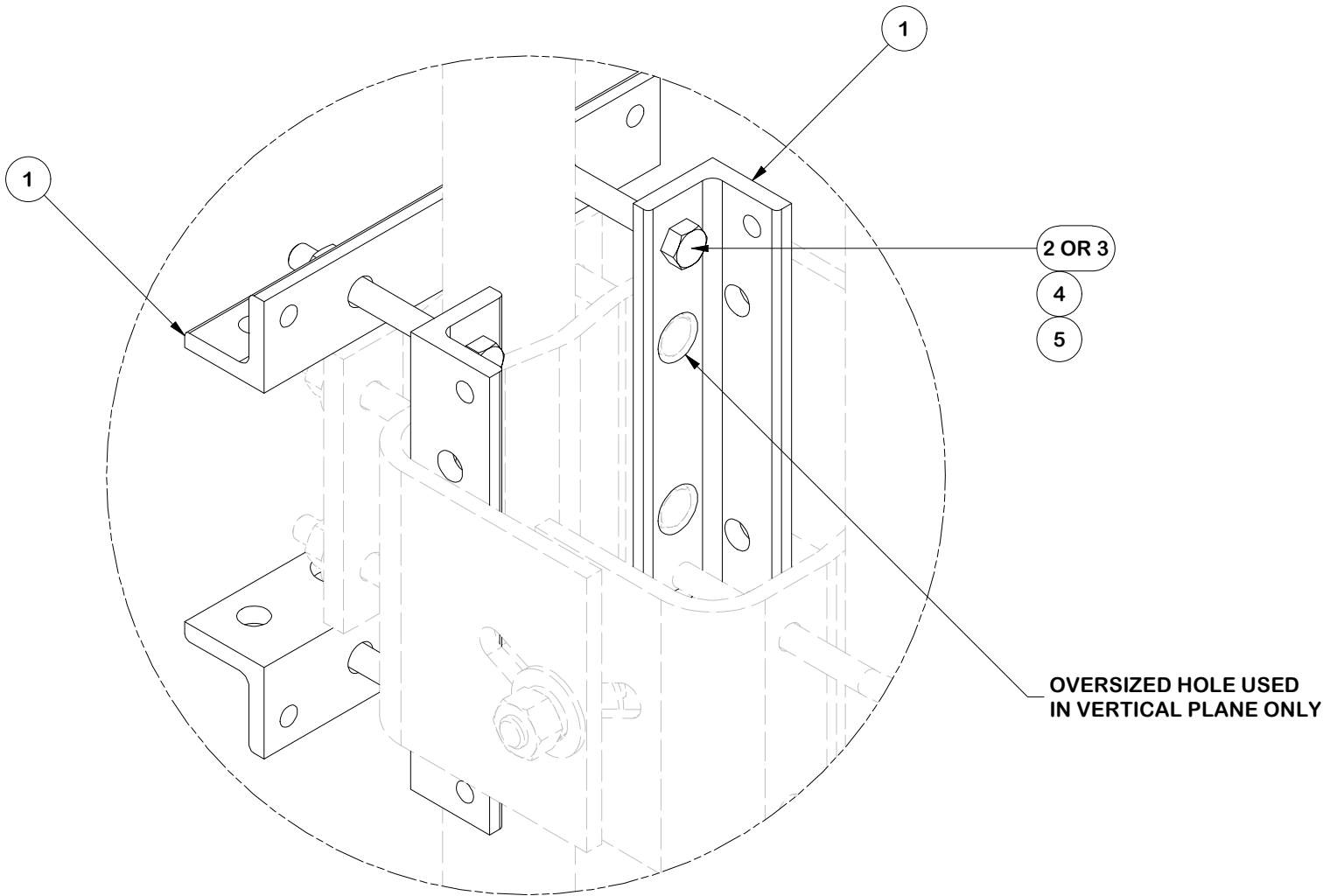
DETAIL A
