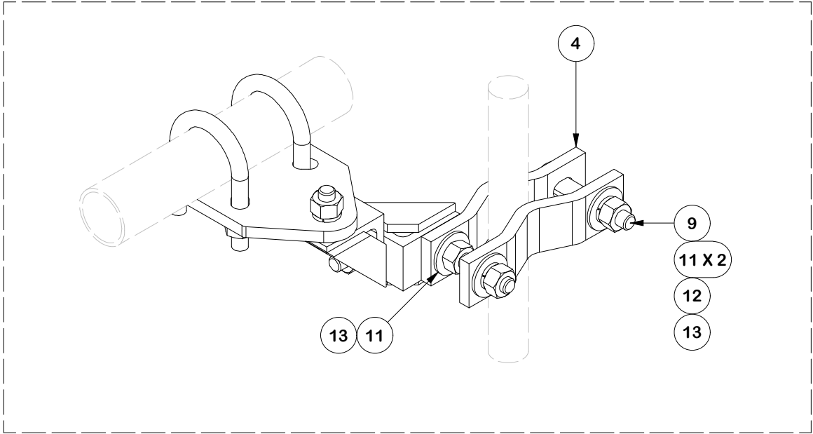
SMALL LEGS 1-1/2" TO 2-3/8" NOTE: FLIP HALF BACK CLAMP
