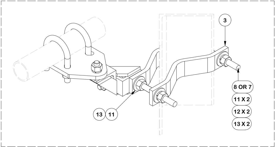
LARGE LEGS UP TO 6" 90 DEG. 8" 60 DEG NOTE: FLIP HALF BACK CLAMP
