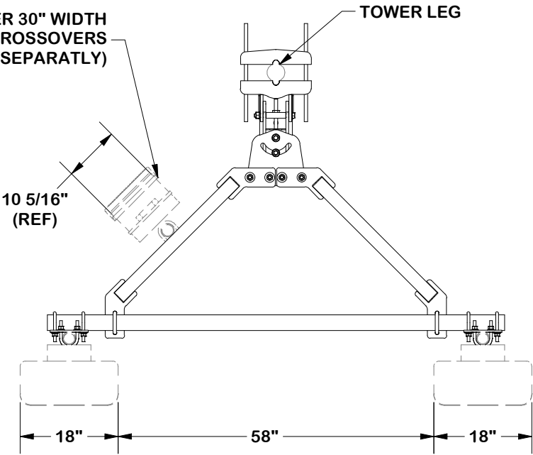
TOP VIEW
