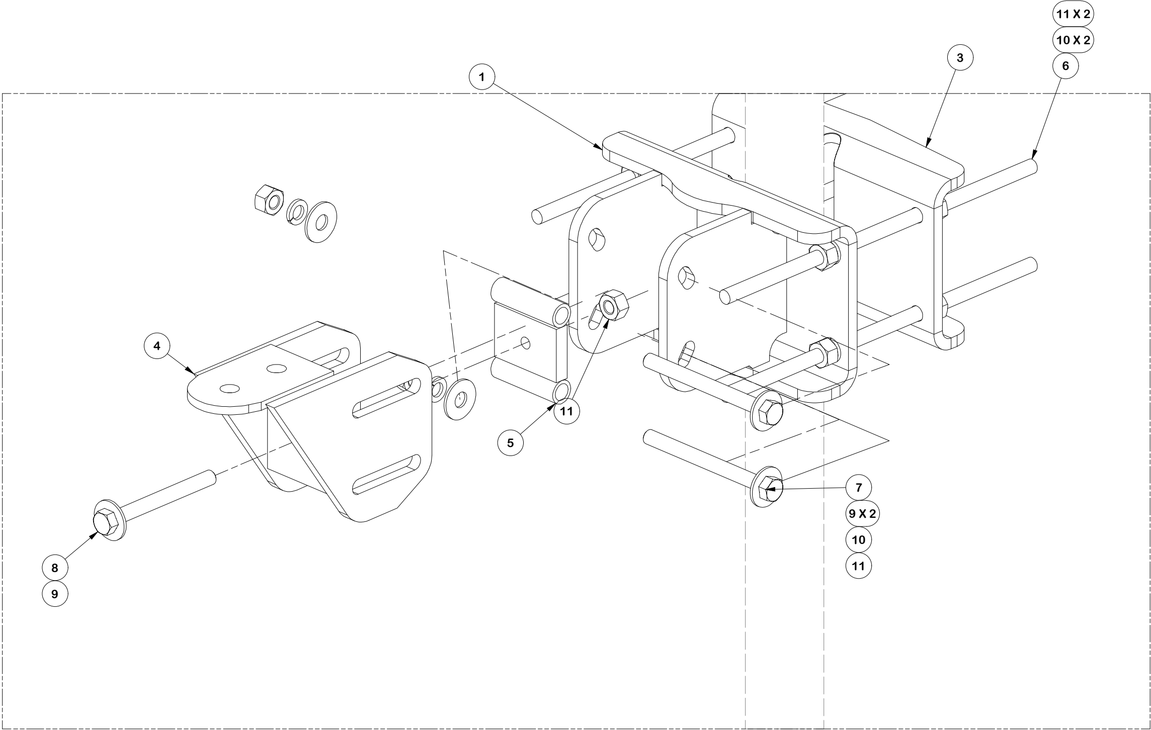
VIEW A
